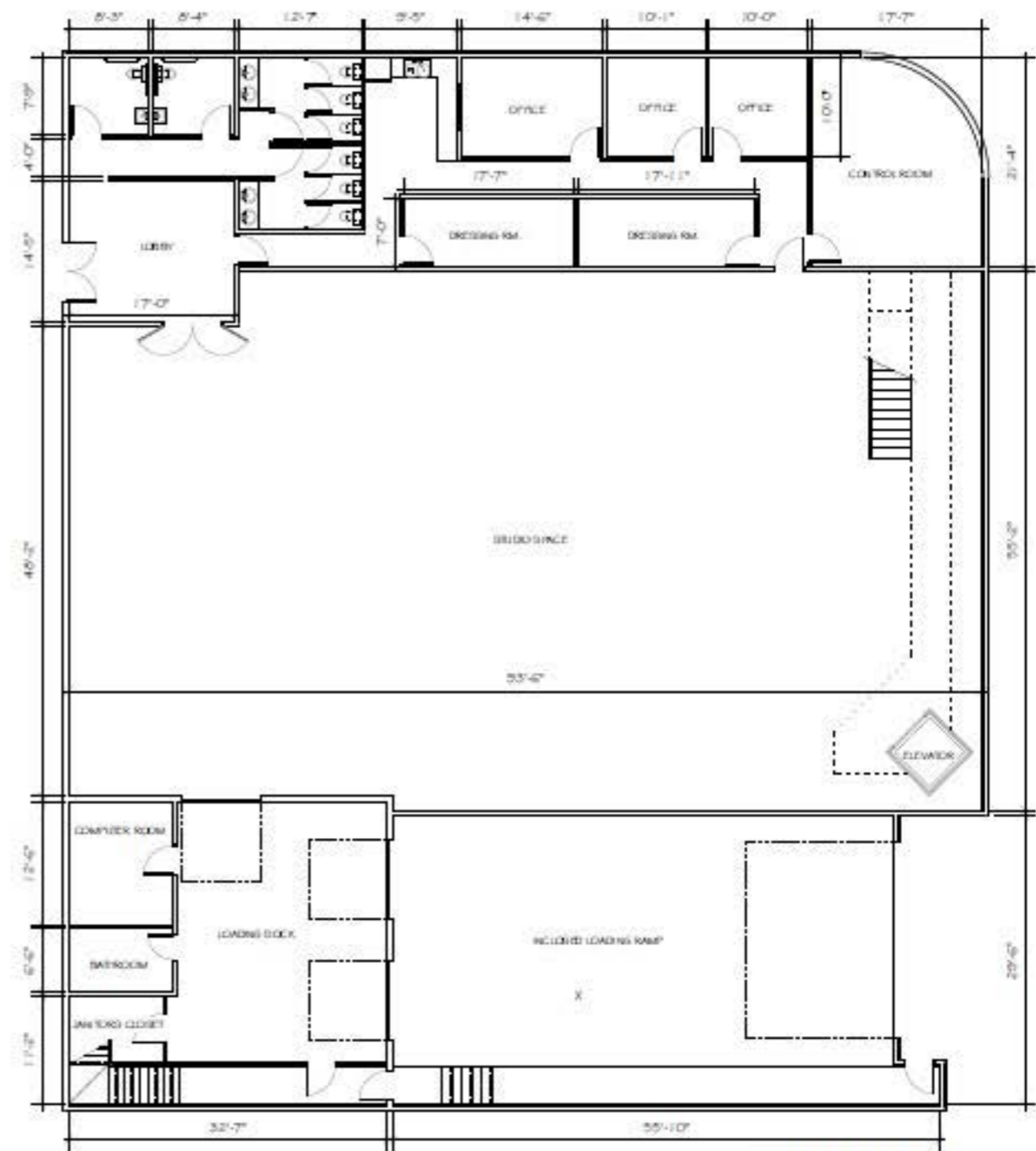
LOWER FLOOR PLAN SCALE: 1/8" = 1'-0"
