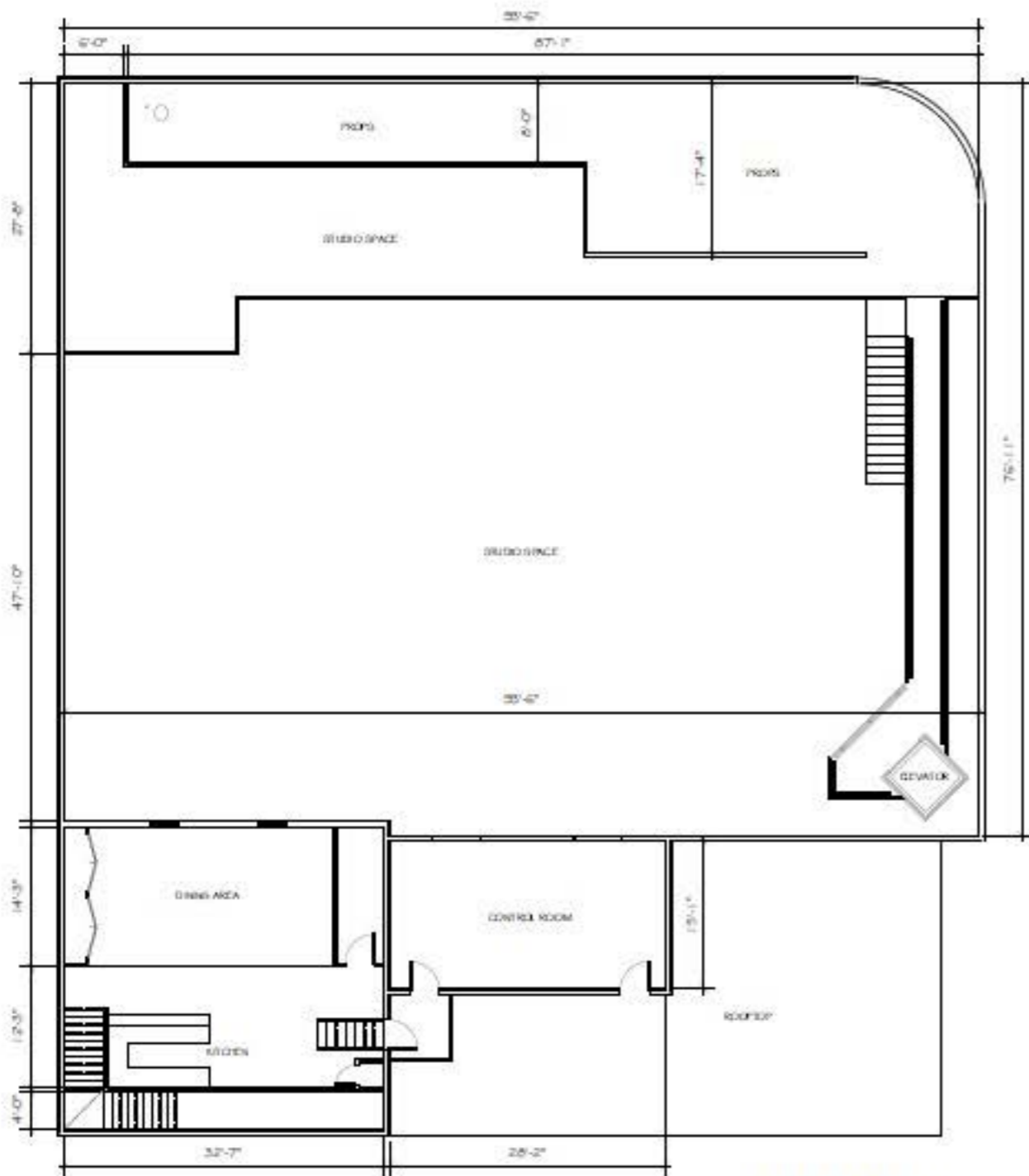
UPPER FLOOR PLAN SCALE: 1/8" = 1'-0"
