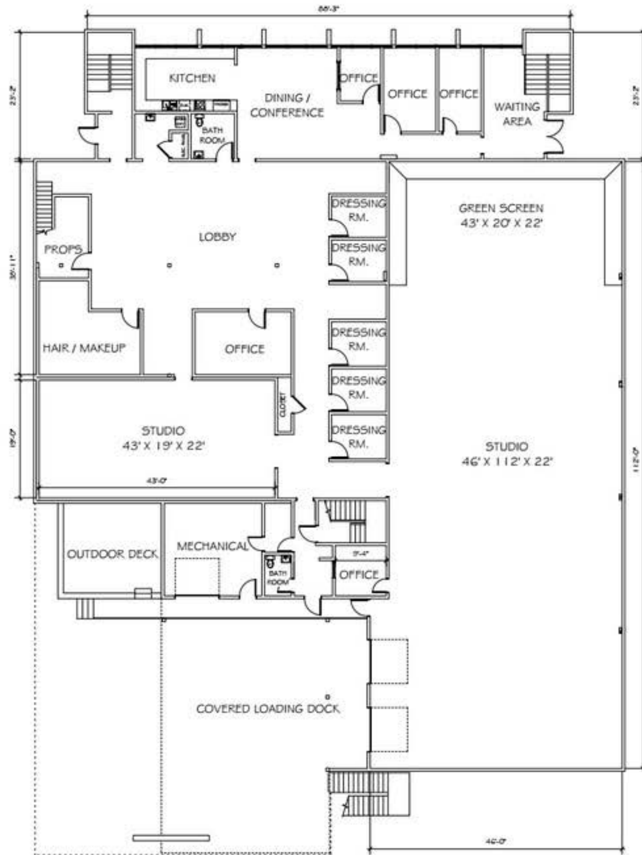
LOWER FLOOR PLAN
